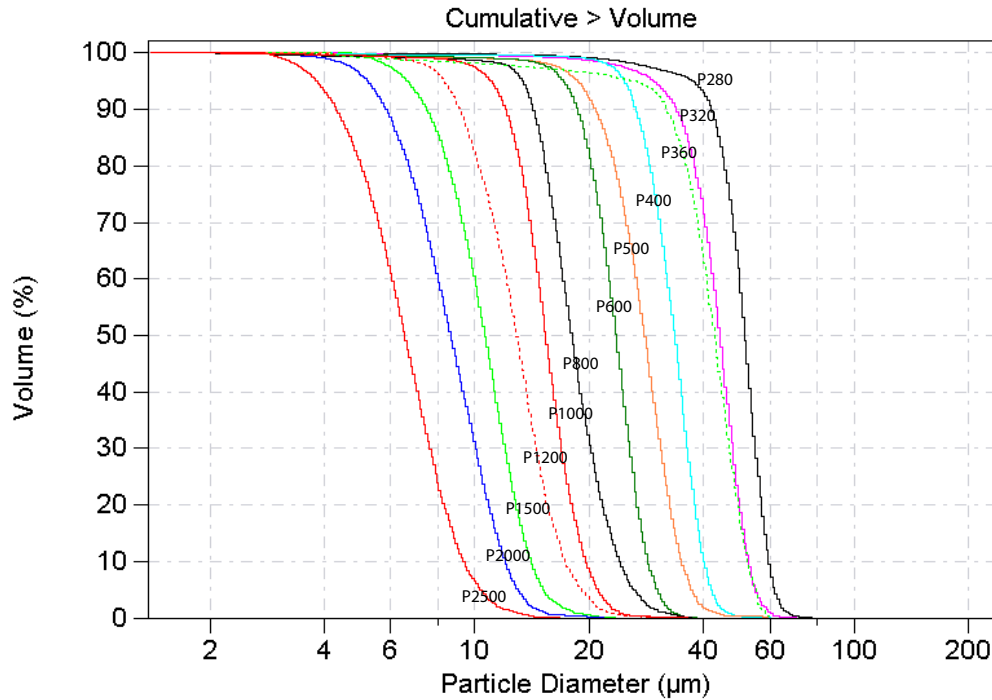
Size Distribution (As per FEPA standard 42-2:2006)
